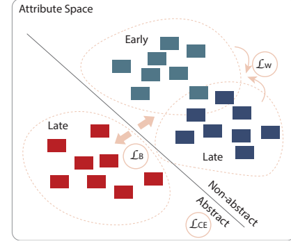
Fig. 3. Illustration of the effects of the three types of loss functions used by DEGA to train the C2A network.
