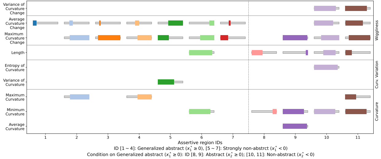
Fig. 8. Quantile Explanation Map (QEM) summarizing the defining conditions of ARs (assertive regions) with IDs 1–11. ARs 1–7 are derived from the first decision tree (for classifying broadly abstract versus strongly non-abstract), while ARs 8–11 are from the second tree (for classifying abstract versus quasi-abstract restricted to broadly abstract streamlines). The predicted majority class for each AR is indicated in the x-axis labels. Each column corresponds to an AR ID, and each row represents one of the nine geometric features of streamlines. A horizontal sliding bar is shown if the feature is involved in defining the AR. The thin gray bar spans the full percentile range (0–100) of that feature across all streamlines, while the colored bar indicates the specific percentile interval used to define the condition for that AR.
