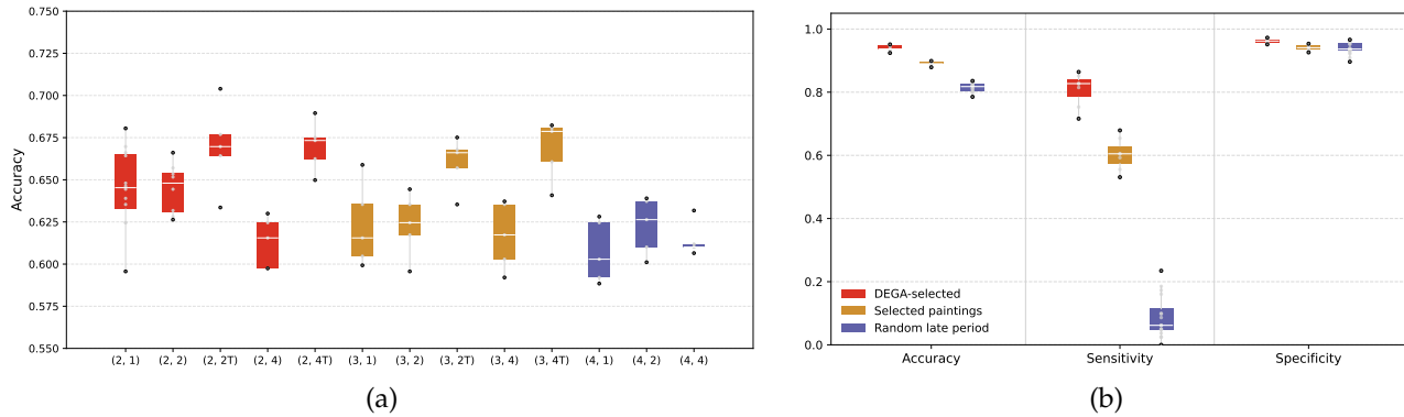
Fig. 4. Classification performance of the C2A network under different experimental setups. All metrics are obtained using the LOPO-CV protocol. (a) Boxplots showing classification accuracy for distinguishing early versus late periods. Each boxplot corresponds to a specific structural configuration of the C2A network, determined by the hyperparameters (d', K) —the dimensionality of the extracted features and the number of LS-classes—as indicated on the x-axis labels. When the Transformer model is used as G_c , the corresponding x-axis label is marked with “T”. (b) Boxplots of accuracy, sensitivity, and specificity for the C2A network with configuration (d', K) = (2, 1) in the task of classifying abstract ( Z = 1 ) versus non-abstract ( Z = 0 ) patches. Three sets of Z labels are evaluated. In the first set, Z labels are generated by DEGA (“DEGA-generated”); in the second, Z labels are assigned as 1 for all flower patches in eight selected paintings based on the result of DEGA (“Selected paintings”); in the third, Z = 1 is assigned to randomly selected patches from late-period paintings (“Random late period”). These three cases are distinguished by color, as indicated in the legends. Across all three label sets, the same proportion \gamma = 0.37 is maintained, that is, 81 late-period flower patches are labeled with Z = 1 . Overall, 85.4% of all patches in the dataset are labeled as Z = 0 . The mean performance measures for the three cases, in the order of “DEGA-generated,” “Selected paintings,” and “Random late period,” are as follows: accuracy: (0.940, 0.891, 0.814); sensitivity: (0.808, 0.603, 0.087); specificity: (0.962, 0.941, 0.938).
